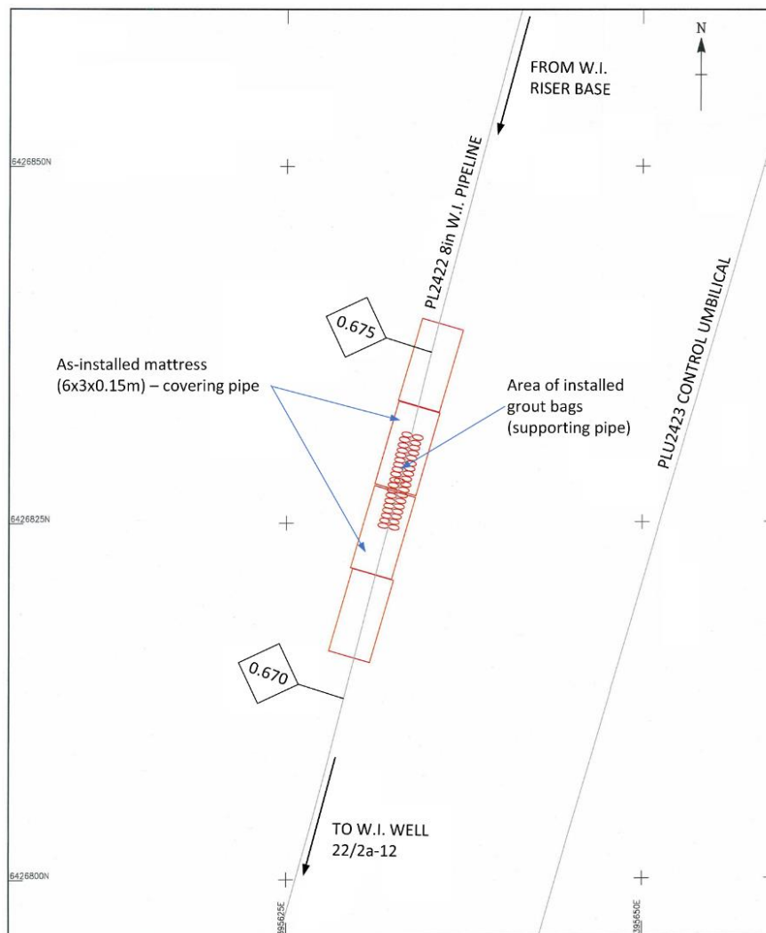
Figure 2.4.5: Span rectification work on PL2422 in 2010
